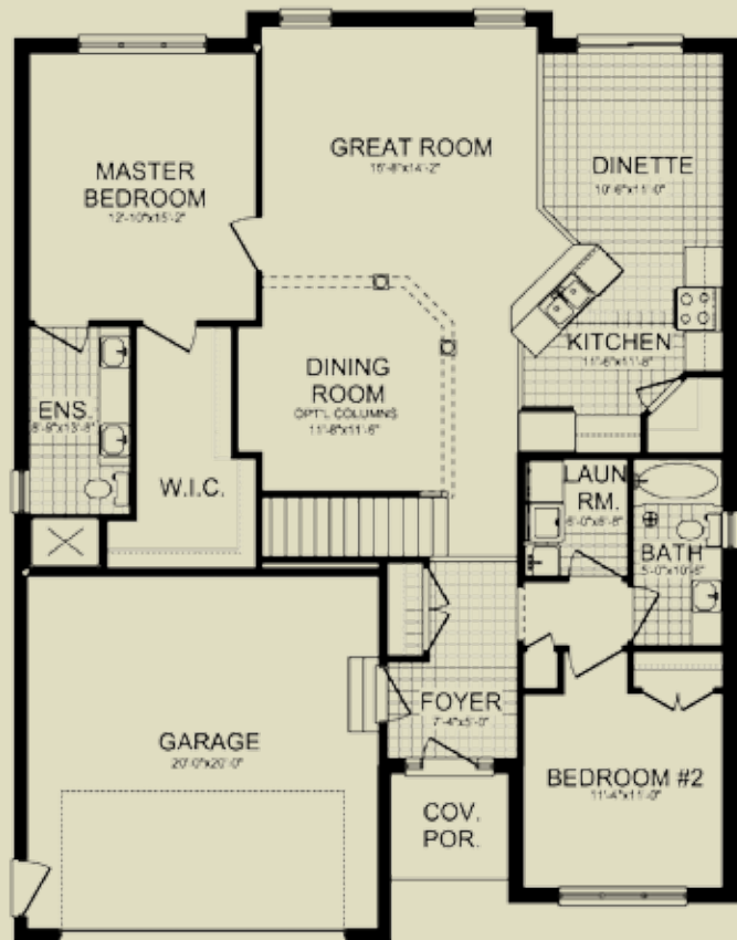
MAIN FLOOR PLAN ELEVATION "A" MAIN FLOOR PLAN WITH 3 PIECE ENSUITE
