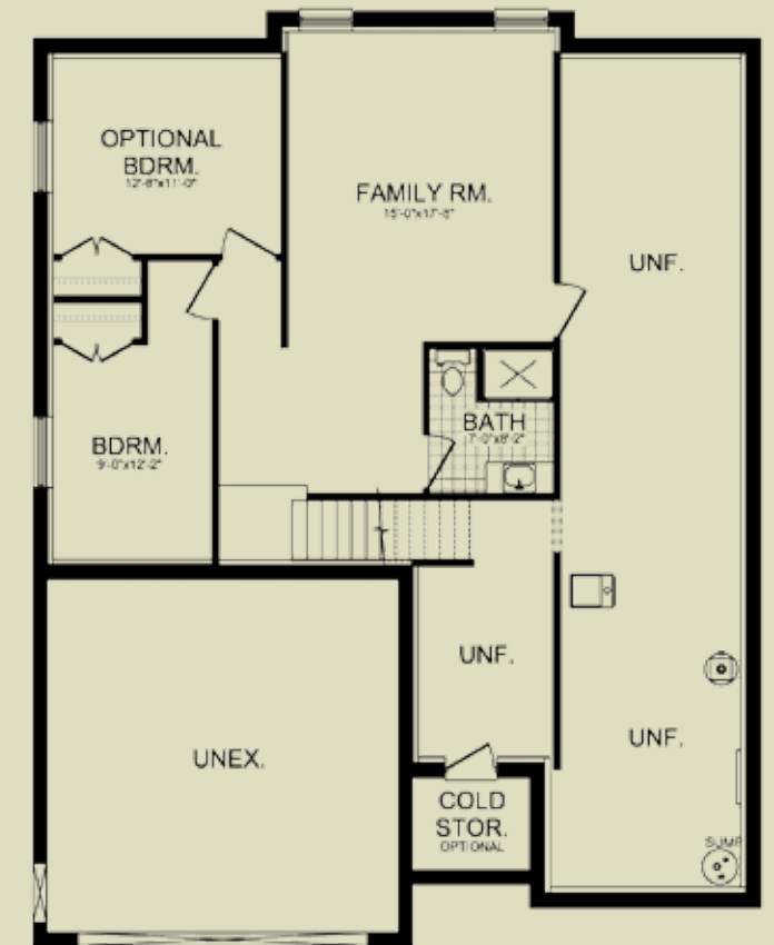
BASEMENT PLAN ELEVATION "A" or "B" FINISHED BASEMENT OPTIONAL 2ND BEDROOM
