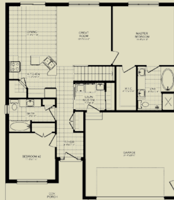
MAIN FLOOR PLAN ELEVATION "B" MAIN FLOOR PLAN WITH 4 PIECE ENSUITE
