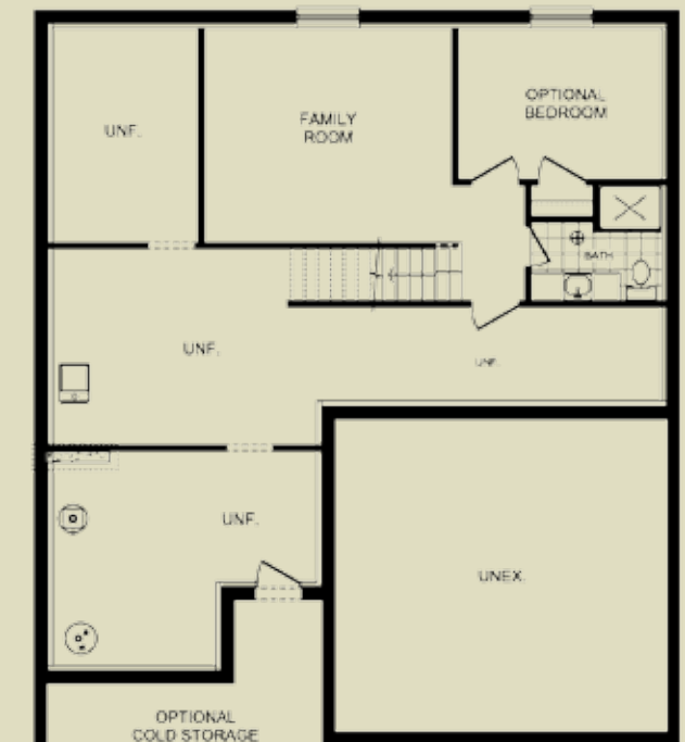
BASEMENT PLAN ELEVATION "B" FINISHED FAMILY ROOM, BEDROOM & OPTIONAL BATHROOM
